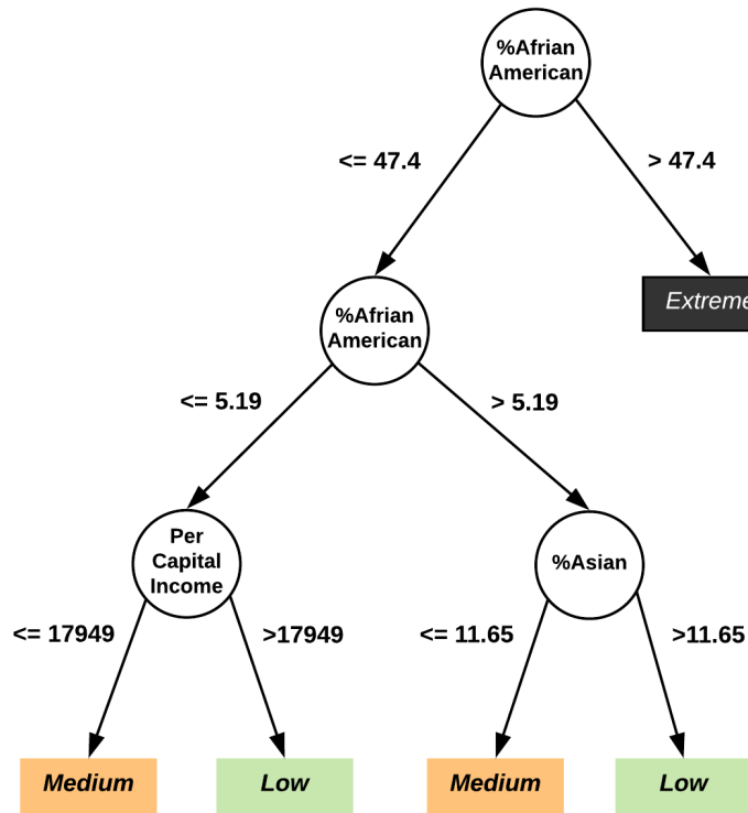
Figure 1. Decision tree with reduced error pruning
