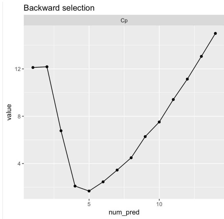
Figure 3. Mallows' Cp with different number of predictors (as can be seen from the graph, #of predictors = 5 gives lowest level of Cp.)
